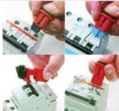
144. Miniature Circuit Breaker Lockout
